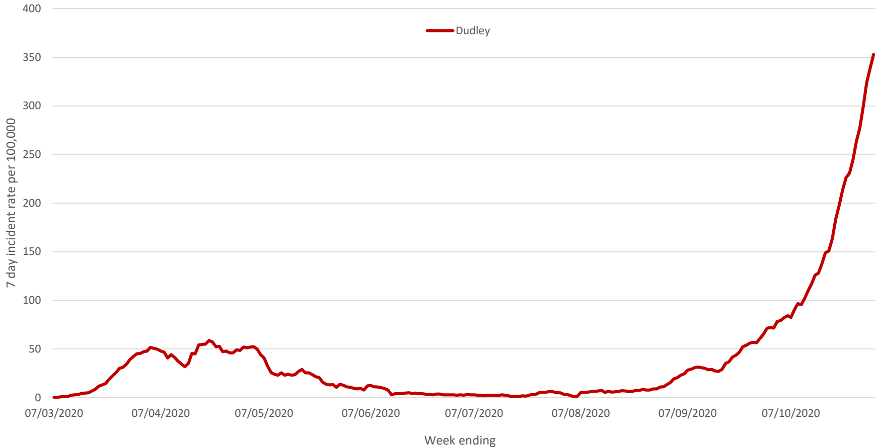
Rolling 7 day Covid Incident Rate Dudley
